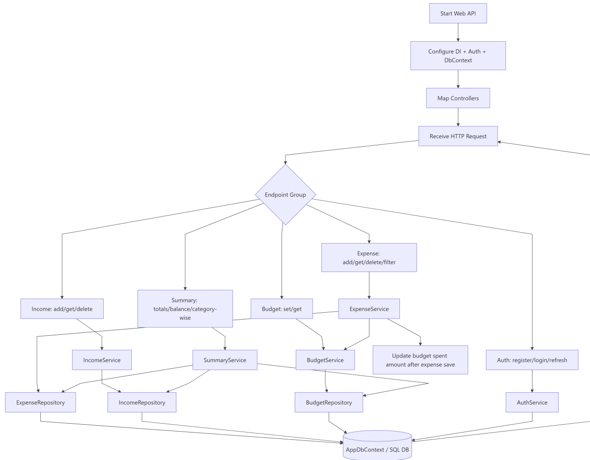
(b) Server flow
