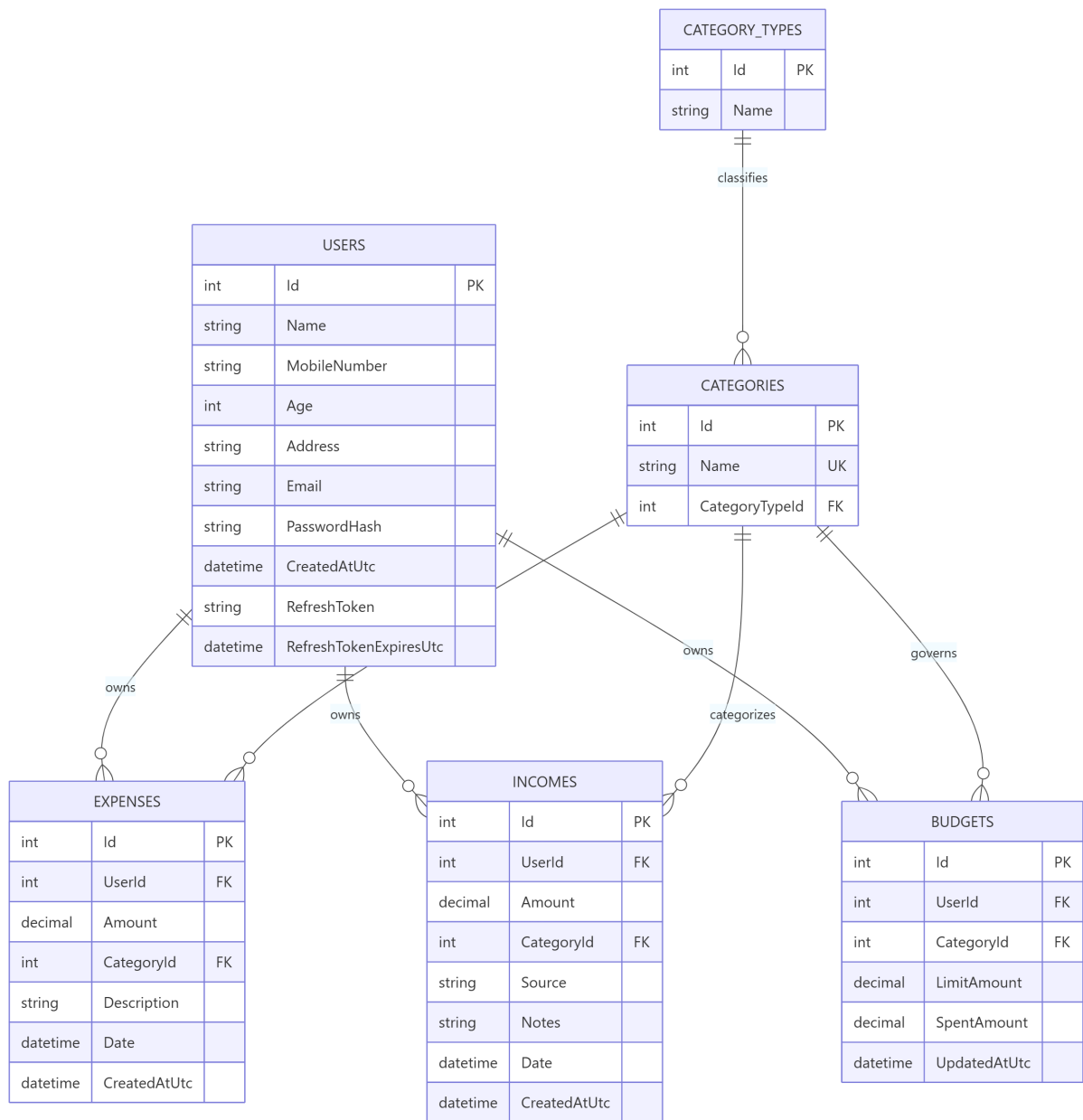
Figure 3: Relational Database Schema Diagram
