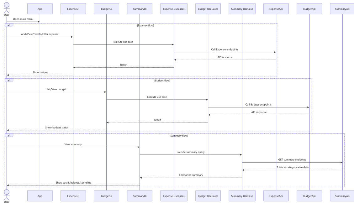
(a) Client interaction sequence
