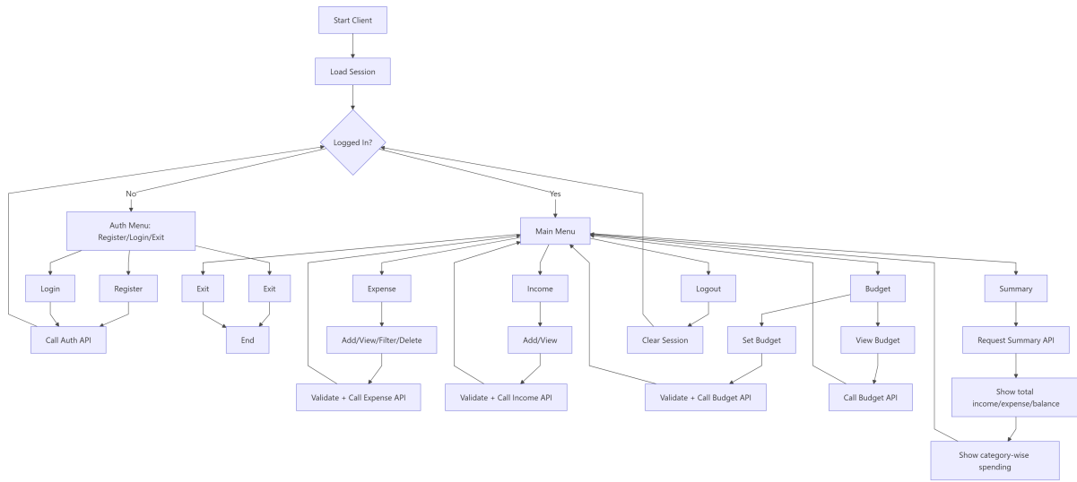
(a) Client flow
